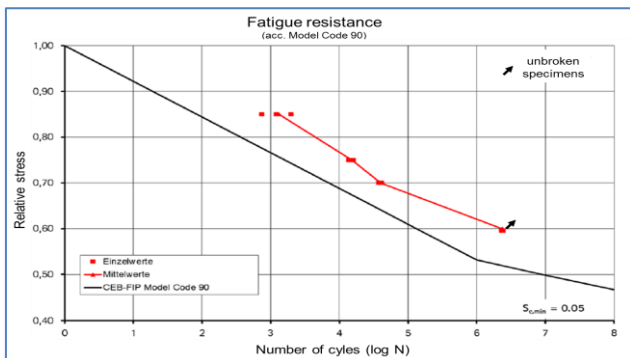
Fatigue resistance measured according CEB-FIB Model Code 90
