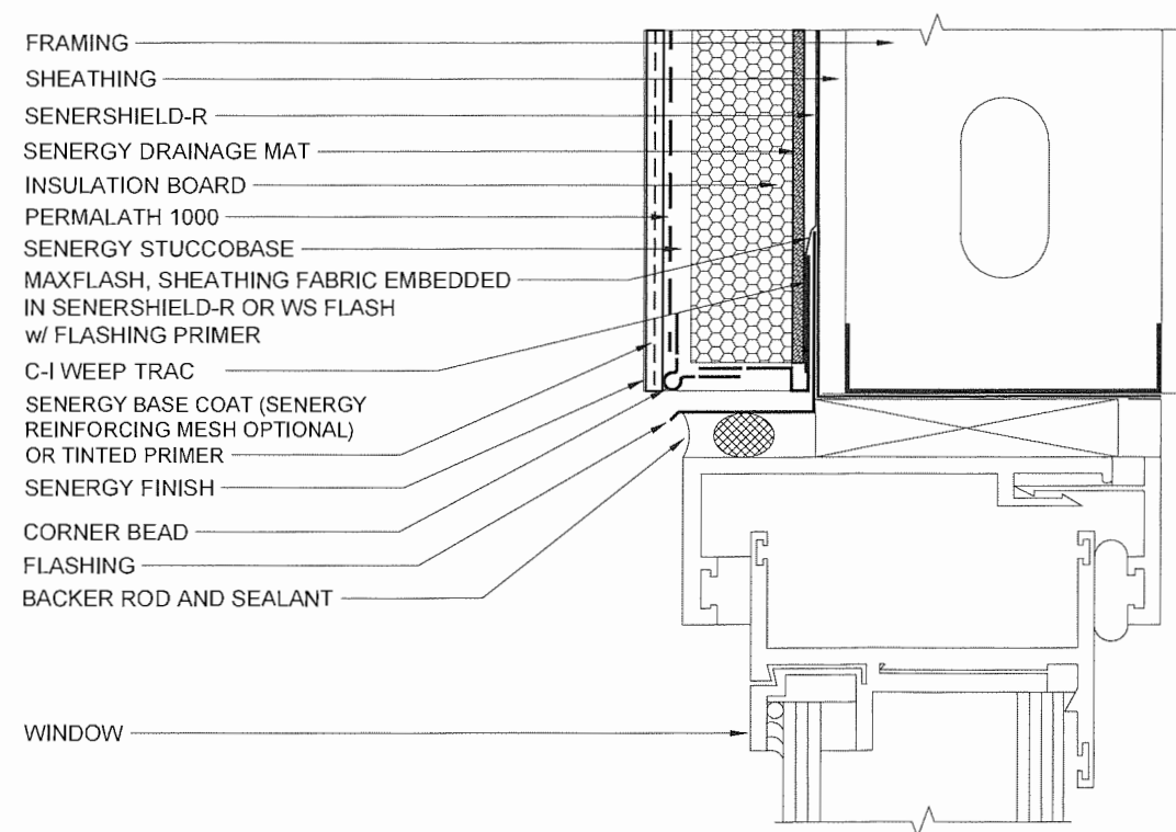
WINDOW HEAD (FLUSH)
