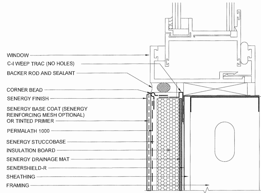
WINDOW SILL DETAIL (FLUSH)
