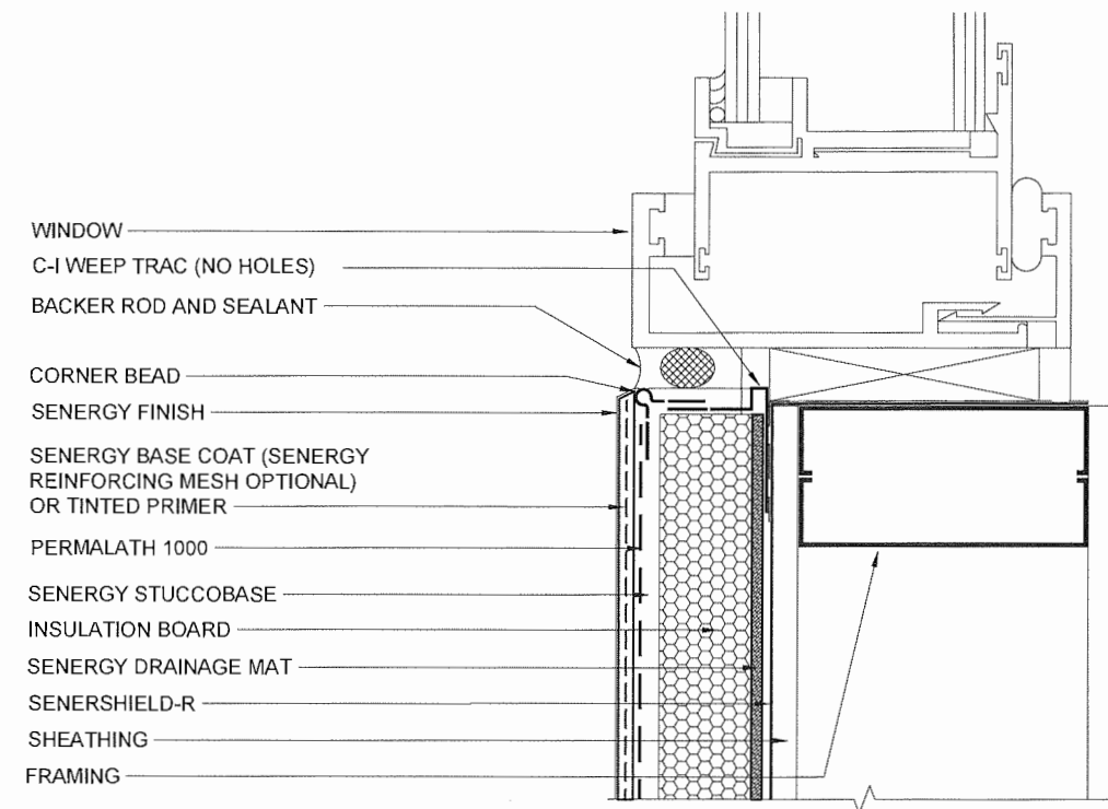
WINDOW JAMB DETAIL (FLUSH)
