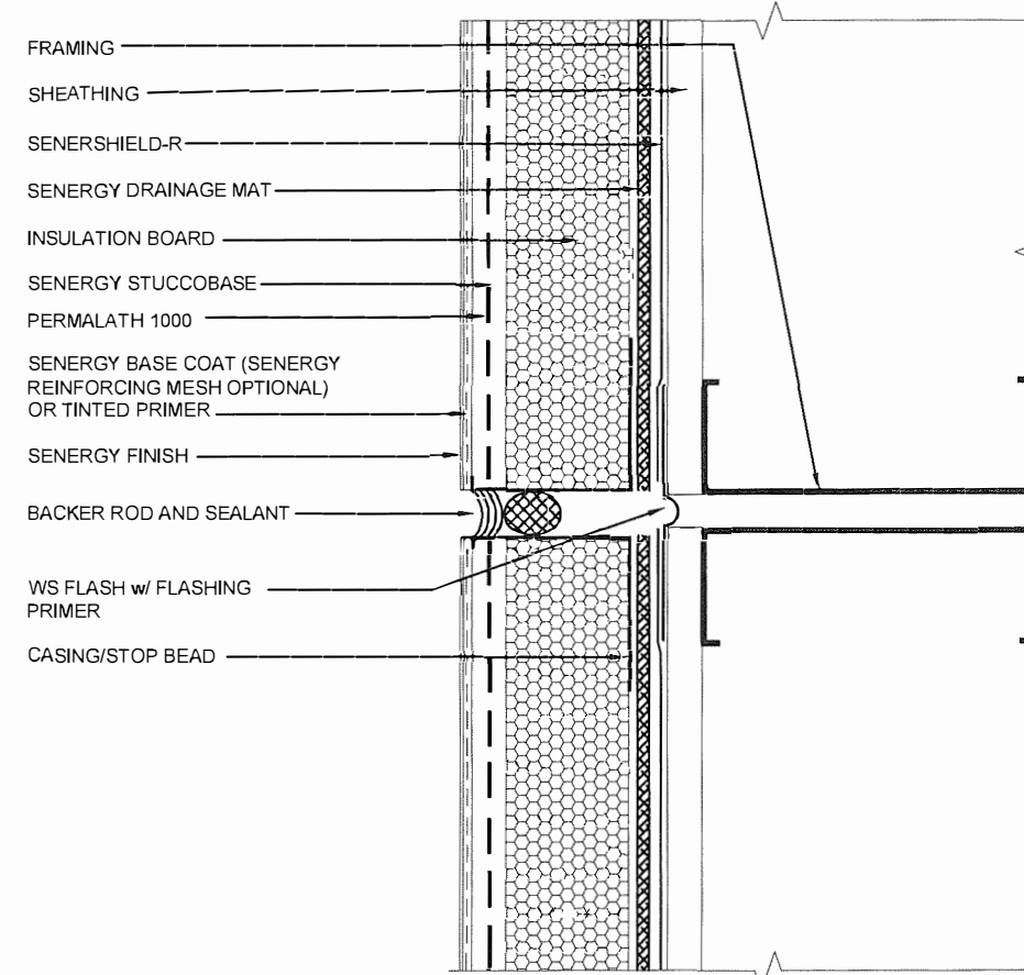
EXPANSION JOINT DETAIL (PLAN VIEW)
