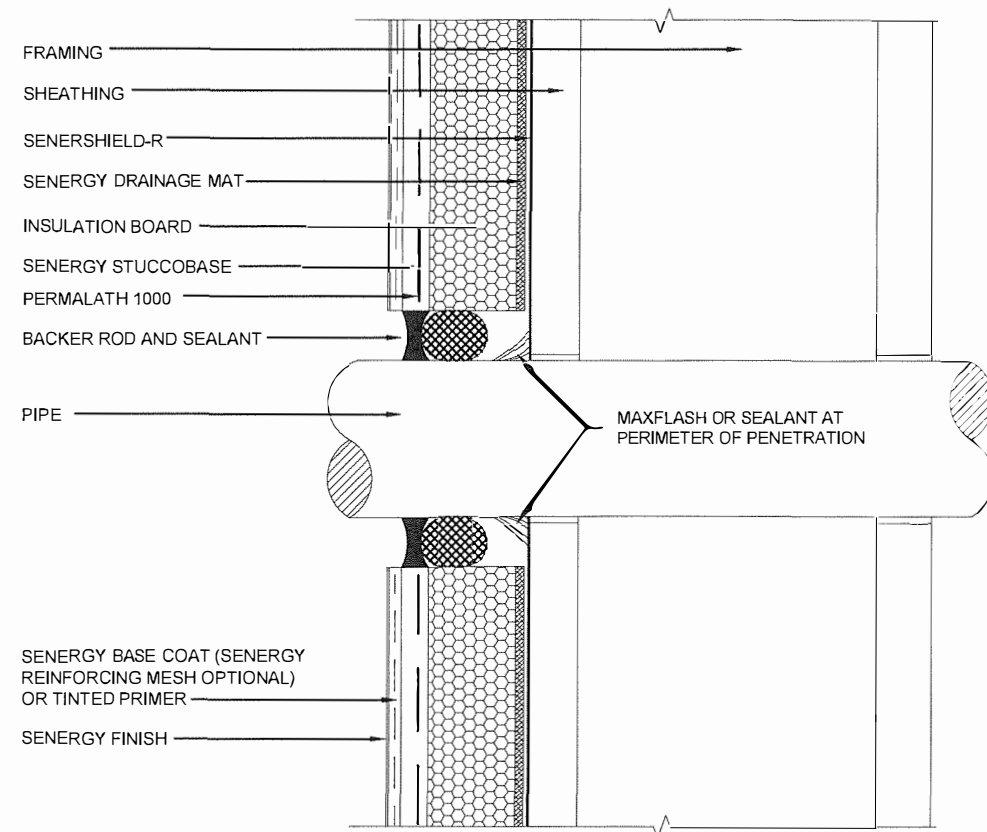
PIPE PENETRATION
