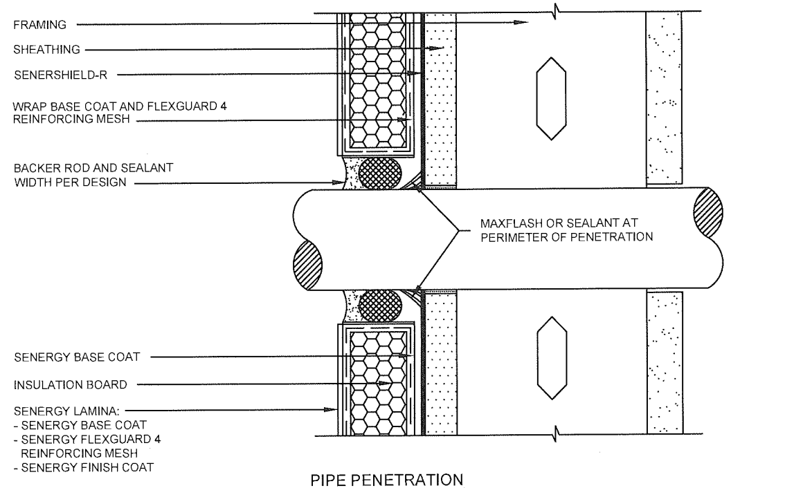
PIPE PENETRATION
