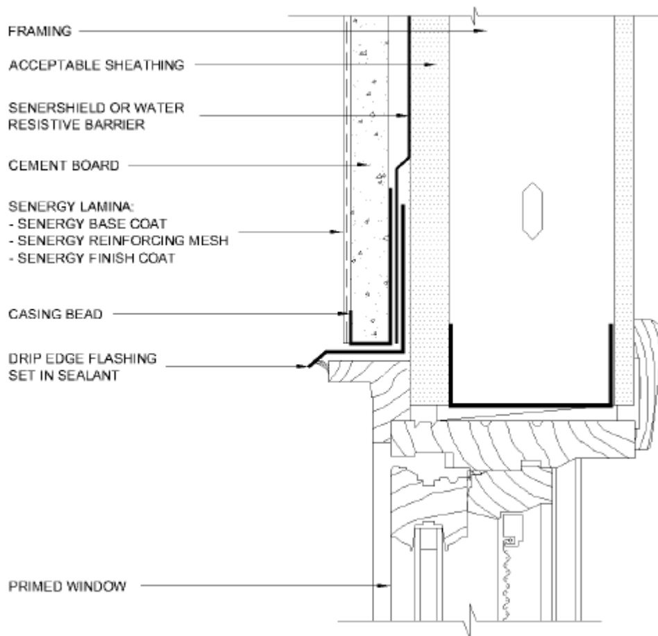
FIGURE 7—TYPICAL PRIMED WINDOW HEAD DETAIL
