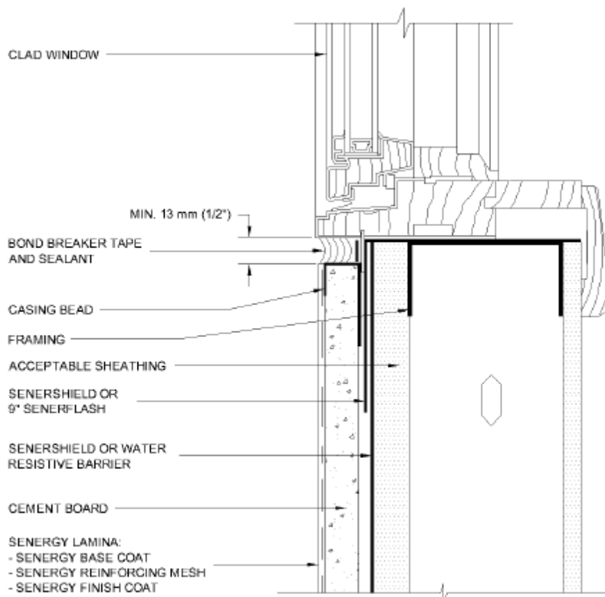
FIGURE 6—TYPICAL CLAD WINDOW SILL DETAIL
