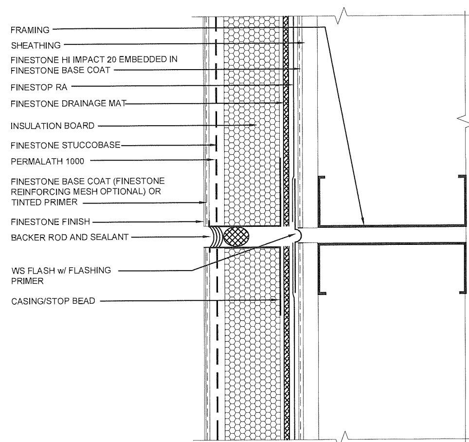
EXPANSION JOINT DETAIL (PLAN VIEW)
