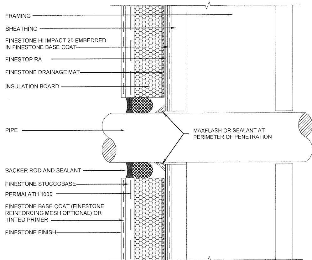
PIPE PENETRATION
