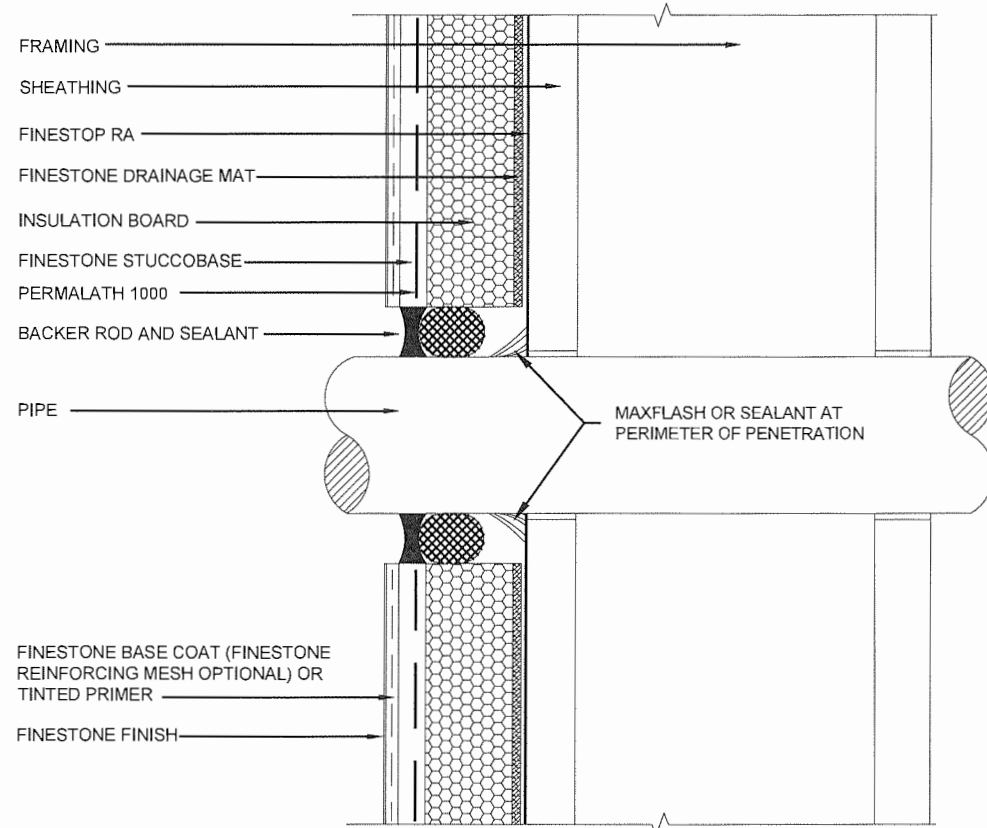
PIPE PENETRATION
