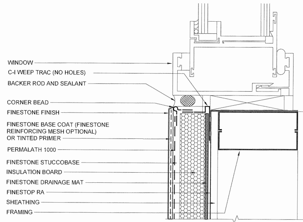
WINDOW JAMB DETAIL (FLUSH)
