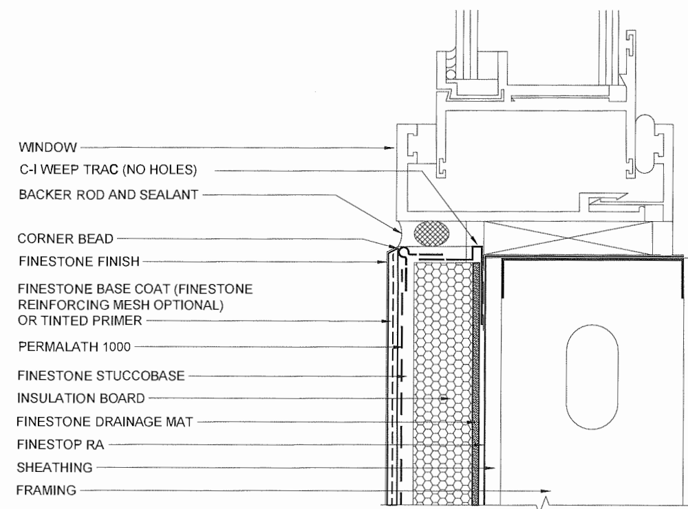
WINDOW SILL DETAIL (FLUSH)
