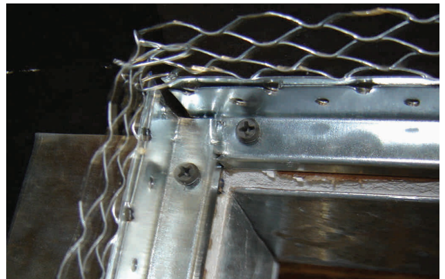
CI Weep Trac Prior to CI Installation
