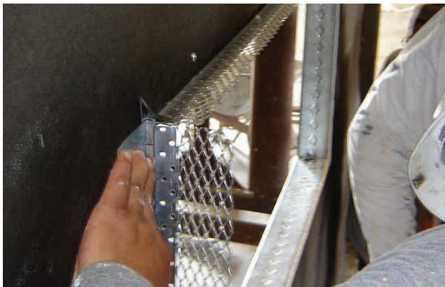
Typical CI Weep Trac at Opening
