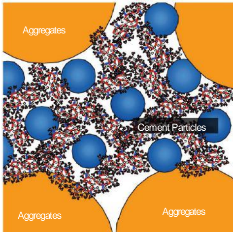
The viscosity of the pore solution is modified by formation of the water envelope and a three dimensional network of the MasterMatrix polymers.
