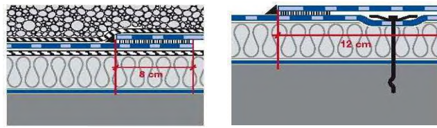
Ballasted roof system
