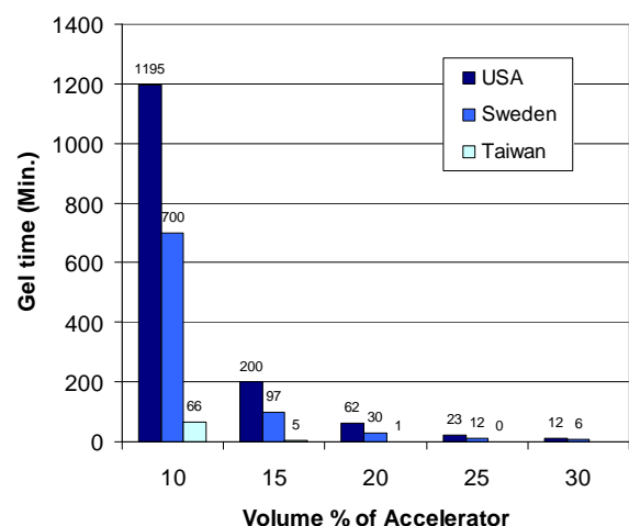
Figure 1: Adjustable gel time with varying accelerator dosage. Values given are at 8°C.
