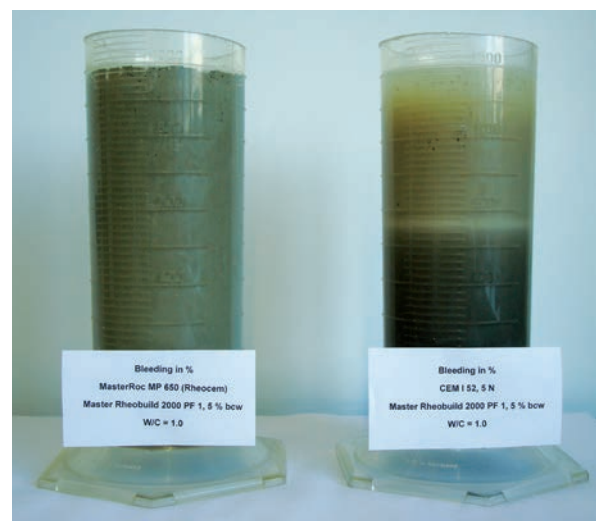
Stable (left) vs. unstable (right) grout
