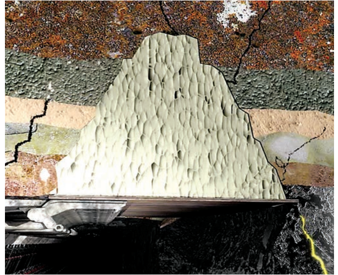
Cavity filling with MasterRoc MP 367 Foam
