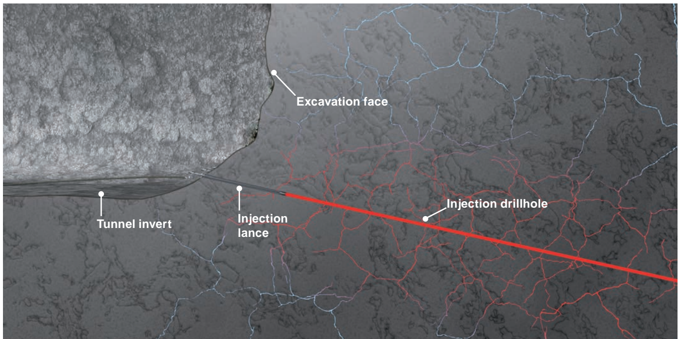
Stable microcement penetrating fine fissures
