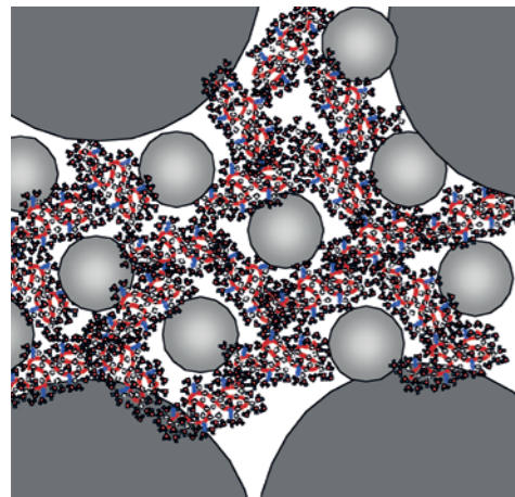
The viscosity of the pore solution is modified by formation of the water envelope and a three dimensional network of the MasterMatrix polymers.
