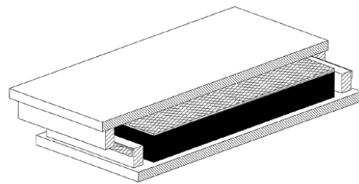
Figure 4: Cross-section of a guided longitudinal bearing (WABO ELASTODEC EL)
