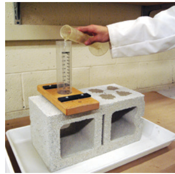
Low pressure permeation and surface puddle retention test
