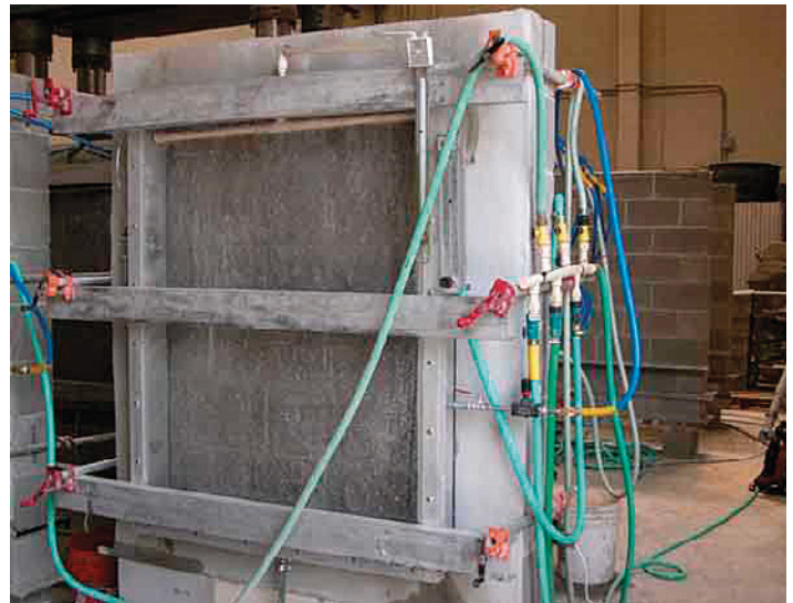
ASTM E 514 Testing of CMU wall
