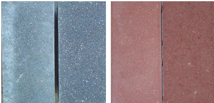
ASTM E 514 Testing of CMU wall
