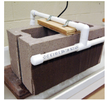
Spray-Bar Tube-test permeation of CMU
